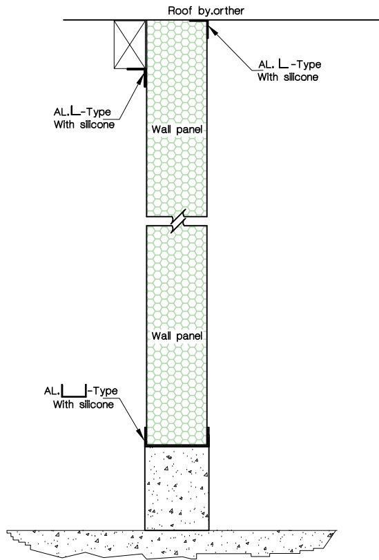
DETAIL ① [ BASE DETAIL ]
