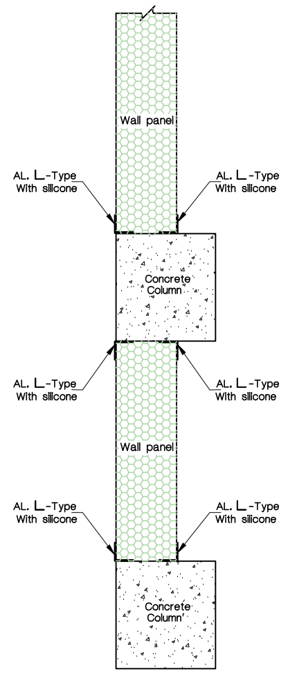
DETAIL ② [ BASE DETAIL ]
