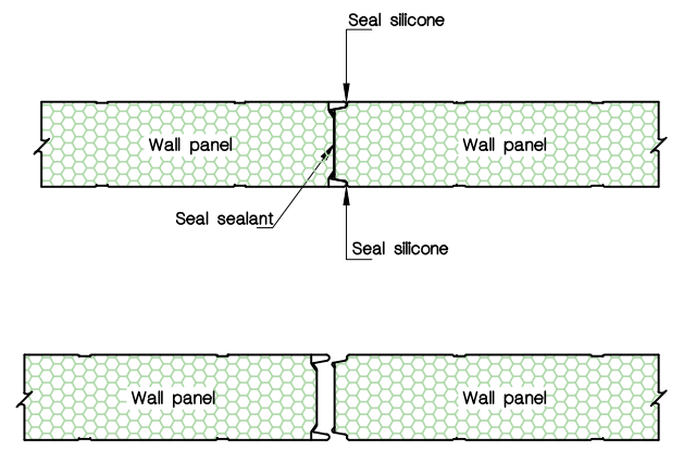
DETAIL ③ [ PANEL TO PANEL , NEW SLIP - JOINT ]
